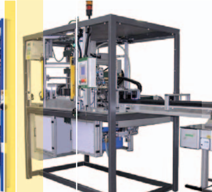
Screw assembly of anti-vibration handles
